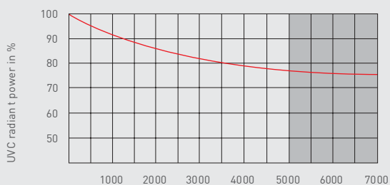
Decrease in UVC radiation for the HNS 55 W G13 HO
