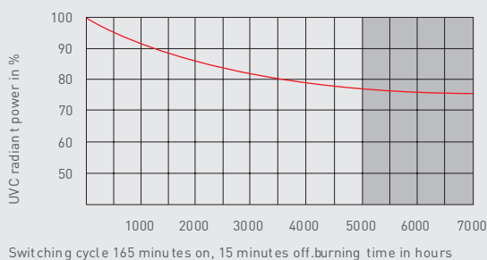
Decrease in UVC radiation for the HNS 55 W G13 HO
